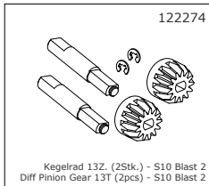
122274 Kegelrad 13Z. (2Stk.) - S10 Blast 2 Diff Pinion Gear 13T (2pcs) - S10 Blast 2
