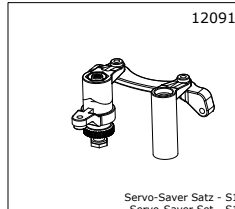
120916 Servo-Saver Satz - S10 Servo-Saver Set - S10
